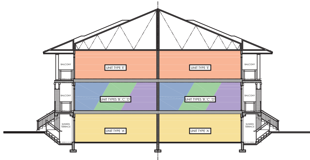
BUILDING SECTION
