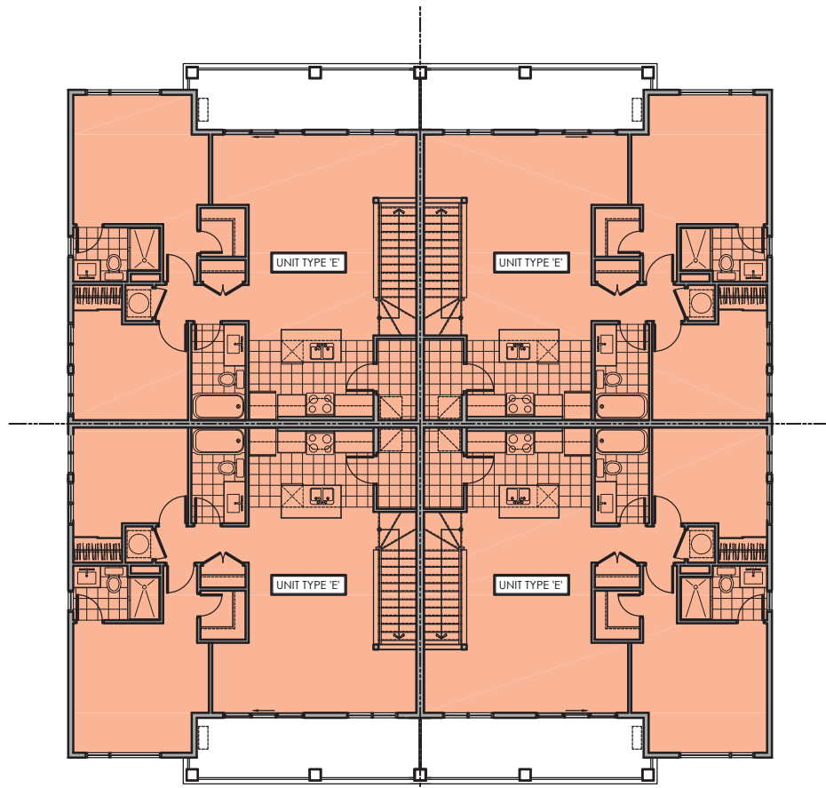
TOP FLOOR
